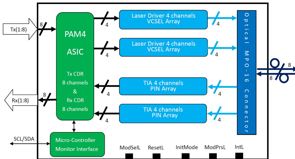
Figure 1. Transceiver Block Diagram
