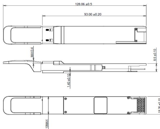
QSFP- DD SR8 MPO 16 Optical Interface Outline
