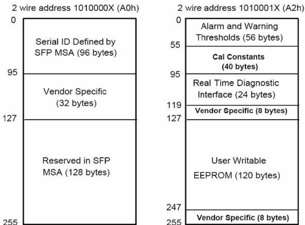
Digital Diagnostic Memory Map (Specific Data Field Descriptions)
