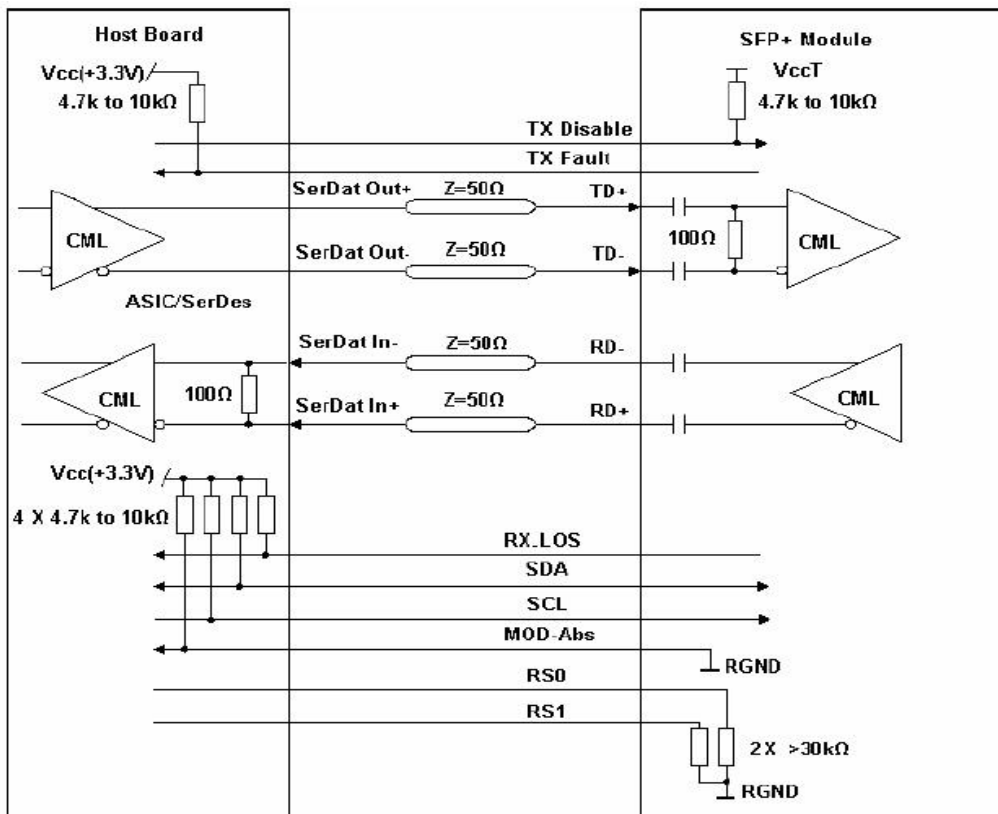
Recommended High-speed Interface Circuit
