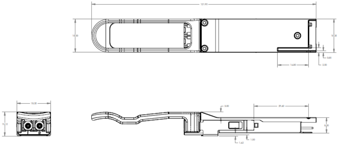
Figure 2 – FTL4S1QE1C mechanical drawing
